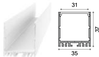
PROFILE 31 mm
