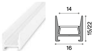
PROFILE 14 mm
