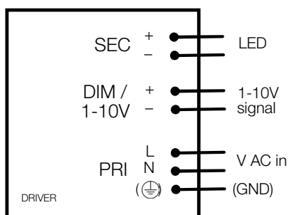
Collegamento 1-10v 1-10V diagram
